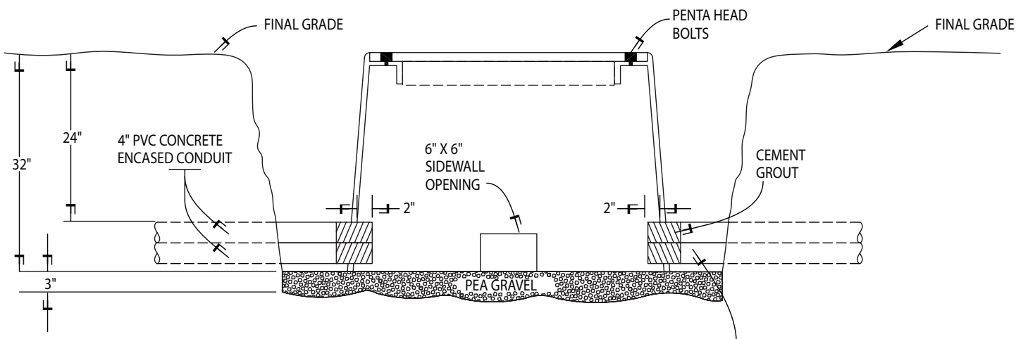
FIBERGLASS SPLICE BOX (MAT'L NO. 12-647) PROVILE VIEW
